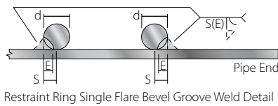
Restraint Ring Single Flare Bevel Groove Weld Detail
