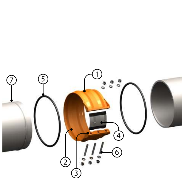
ONE SEGMENT HOUSING
