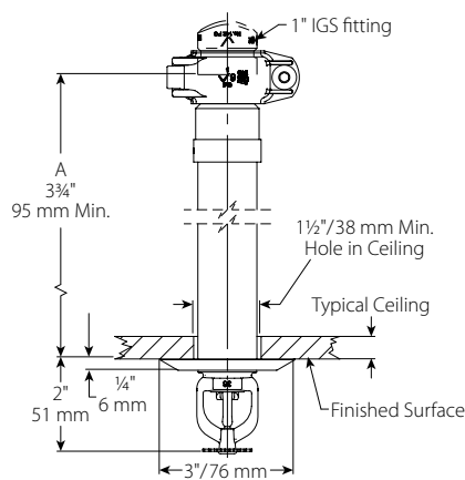
Flush, Grooved V3613, V3615
