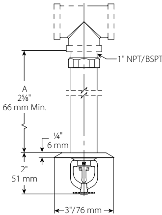
Intermediate, Threaded V3613, V3615
