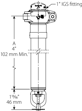
Plain Barrel, Grooved V3613, V3615
