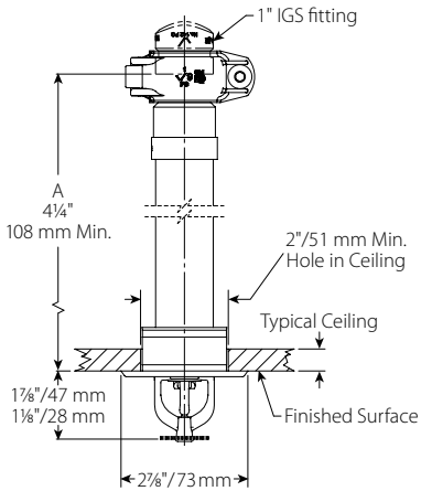
Recessed, Grooved V3613, V3615
