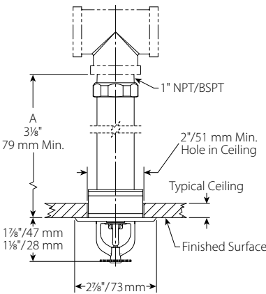
Recessed, Threaded V3613, V3615
