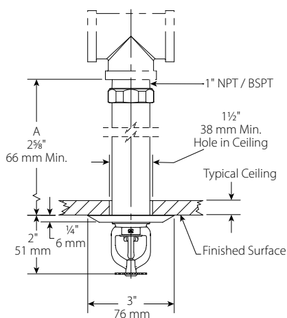
Flush, Threaded V3613, V3615
