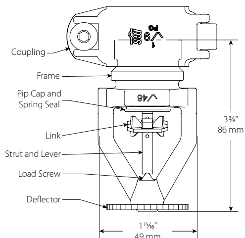
Grooved V4601
