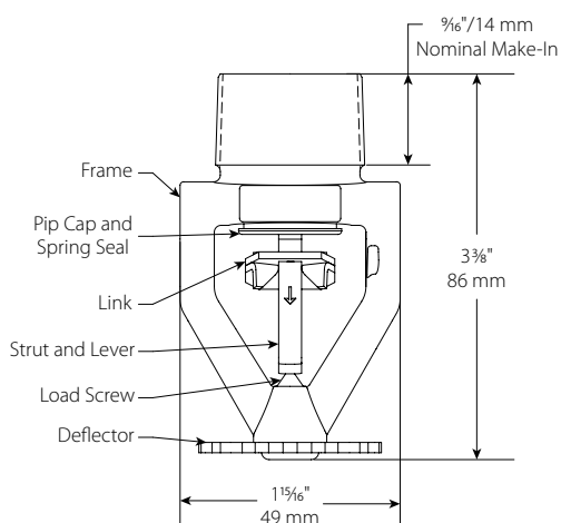
Threaded V4601
