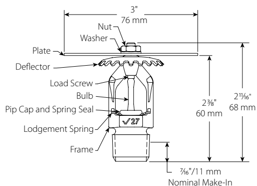
Threaded V2704 Intermediate
