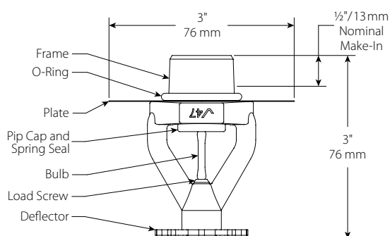
Threaded V4702 Intermediate
