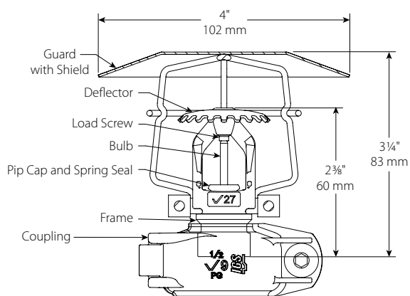
Grooved V2704 Guard with Shield
