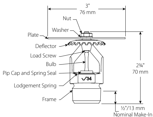
Threaded V3402 Intermediate
