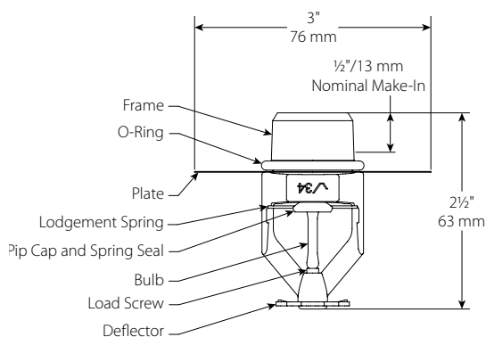
Threaded V3408 Intermediate
