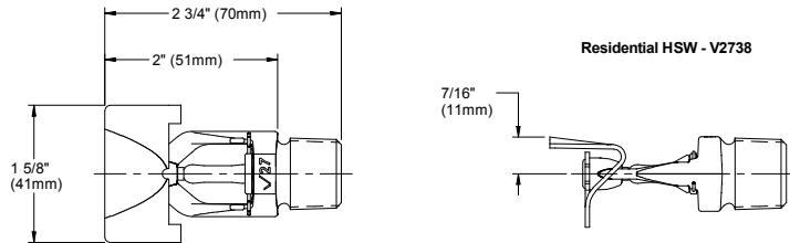
Figure 1 – \frac{3}{4}" Adjustment Recessed – V2738 (drawing not to scale)
