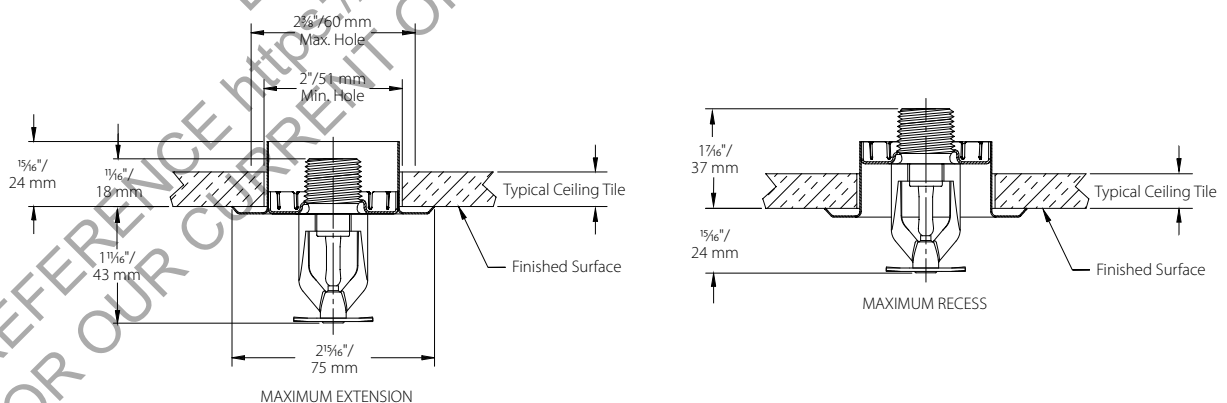
Maximum Recess – 3/4" Adjustment Recessed – V2740 (drawing not to scale)
