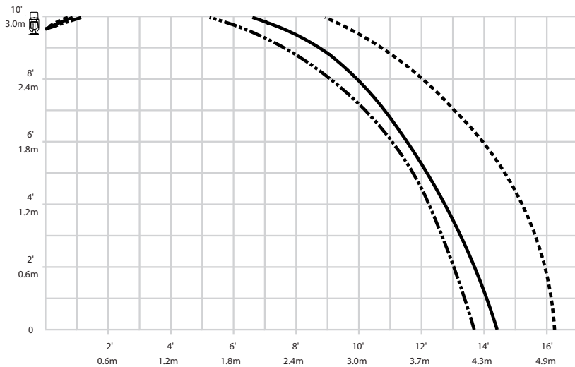
Models V2725, V2726 K80 Conventional Pendent Distribution Patterns – Trajectory
