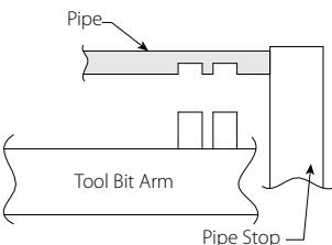
Knife Profile for Double groove Only*
