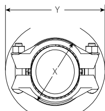
Style 905 Pre-Assembled (Installation-Ready Condition)
