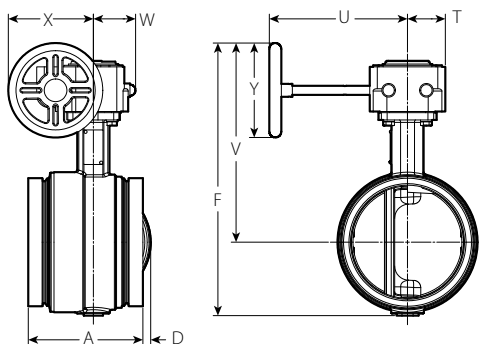
Gear Operator 2 – 6"/DN50 – DN150
