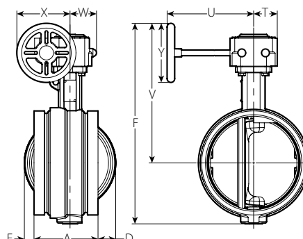
Gear Operator 8 – 12"/DN200 - DN300
