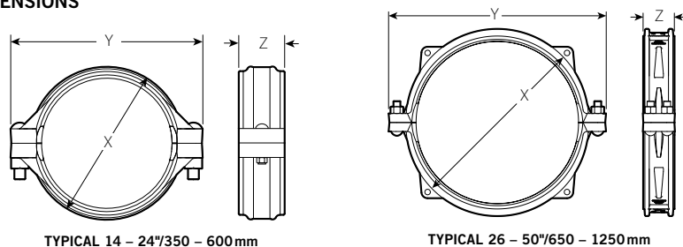
TYPICAL 14 – 24"/350 – 600mm
