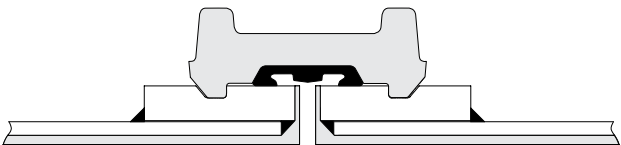
Rubber-Lined Overhung
