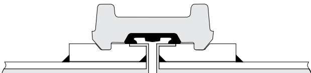
Rubber-Lined Flush
