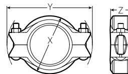
Style SC77 Joint Assembled
