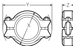
Style SC77 Pre-Assembled (Installation-Ready Condition)
