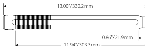
13.0" Straight Reducer
