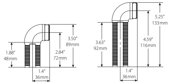
Short 90° Low-Profile Elbow Reducer
