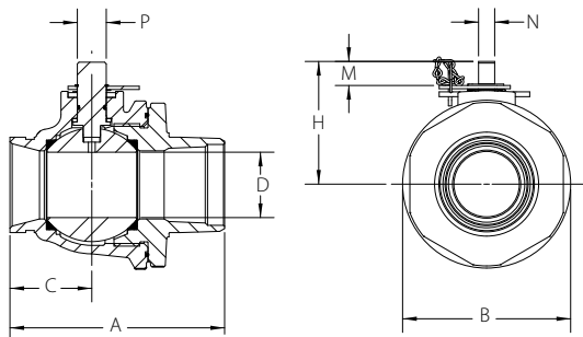
Bare Valve Threaded End 2 – 4"/DN50 – DN100
