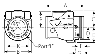
Typical 4"/DN100
